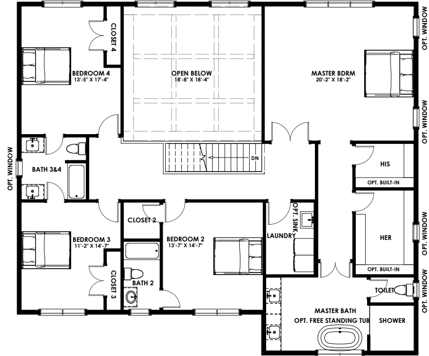
UPPER LEVEL 2,383 SQ FT
